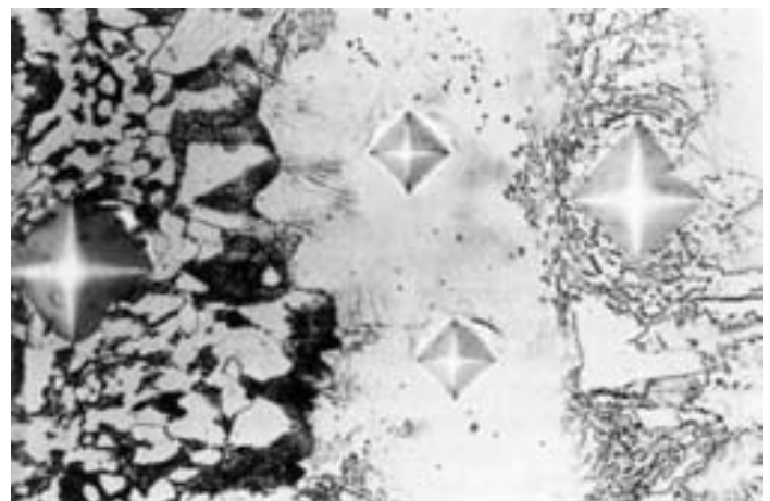
Fig. 3. Welding mild steel with a 308 L electrode. Note the hardness increase (smaller impression from measuring tool) close to the mild steel side.
