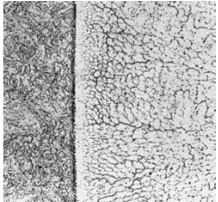
Fig. 6. Weld between 2.3 Cr 1 Mo and 16 Cr 13 Ni Nb steels. Weld metal Inconel. No carburization of weld metal fusion zone area (after approx. 9 000 h at 500 to approx. 600°C). (300x).
