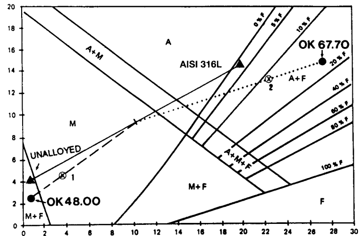
Fig. 1. The Schaeffler-de-Long diagram. The definition of the composition of the weld metal when welding stainless steel to unalloyed steel. In the derivation of these compositions (point 1 and 2) has been assumed that the weld metal is diluted by equal amounts of each of the base materials. (AISI 316L and unalloyed steel) and that 70% of the weld metal is made up of the consumable. Point 1 illustrates the use of an unalloyed consumable (OK48.00) and point 2 illustrates the use of a suitable over-alloyed stainless consumable (OK 67.70).
